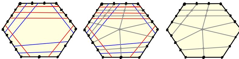
FIGURE 2. The two systems of dual curves in C are indicated on the left, the dual of \Gamma is indicated in the middle, and the \mathcal{VH} -subdivision C' is indicated on the right.
